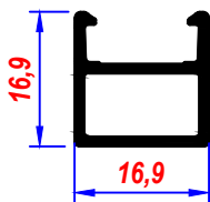
ALM. PRF. 610 cm
