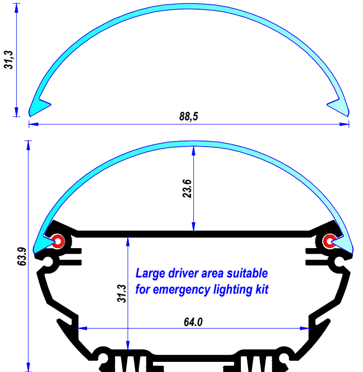
YA-P01 A PC. Diffuser Opal - Transparent
