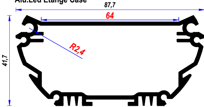
YA-P01 B Alu. Laser End Cap Light Gray
