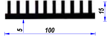
YA-596 Alm. Sğt. Prf.
