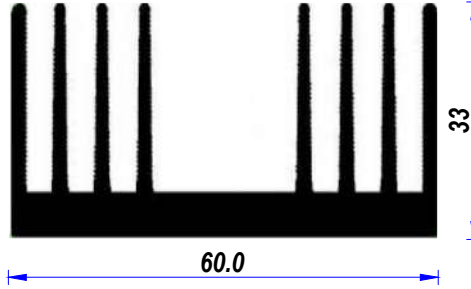
YA-598 Alm. Sğt. Prf.
