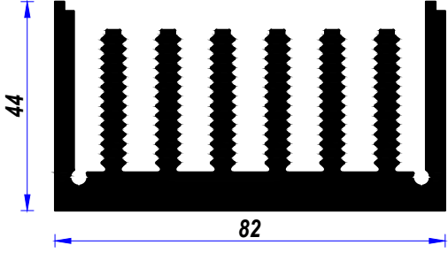
YA-583 Alm. Sğt. Prf.
