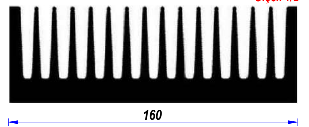
YA-598 Alm. Sğt. Prf.
