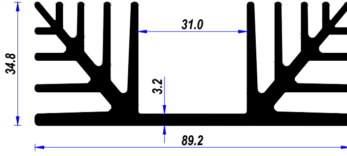
YA-592 Alm. Sğt. Prf.
