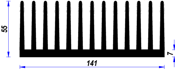
YA-601 Alm. Sğt. Prf.
