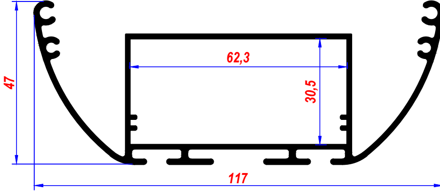
YA-208 Alu.Led Etange Case
